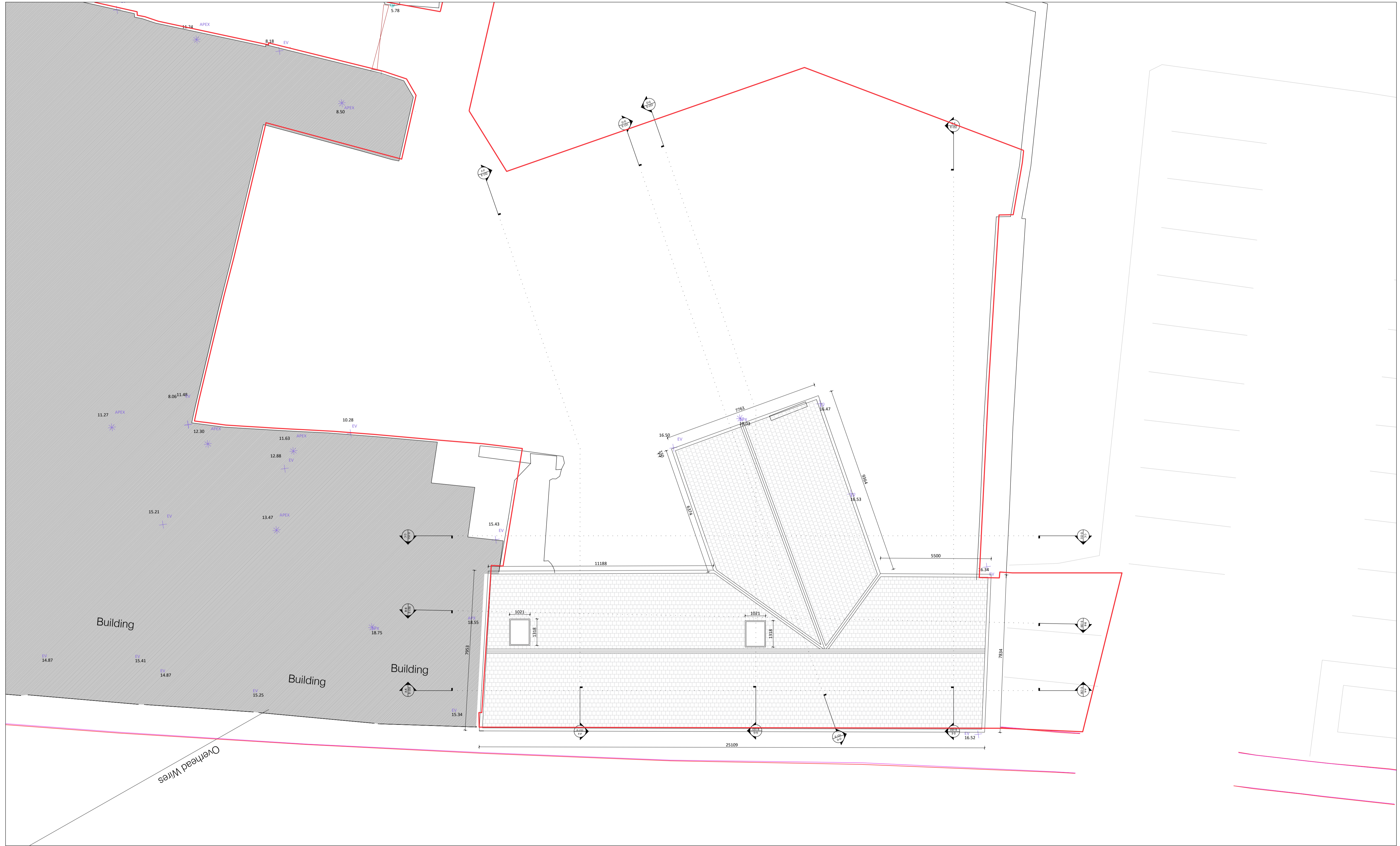
01 Roof Plan As Existing Scale: 1:100
